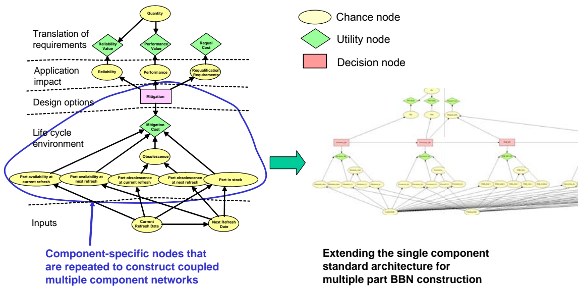
Figure 4. Example Bayesian Belief Network (BBN) for determining whether to replace or not replace electronic components at a specific re-design point.
