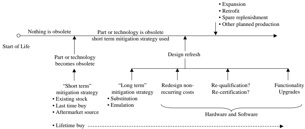
Figure 1. Timeline of events managed in the MOCA design refresh planning tool.
