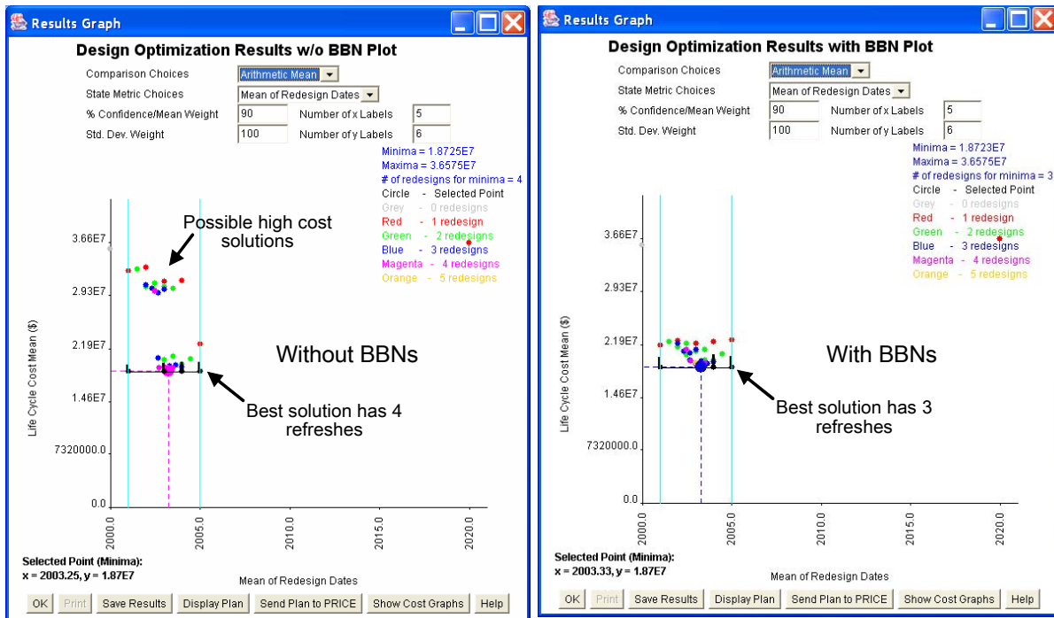
Figure 5. Results for the analysis with (right) and without (left) a BBN used to make part replacement decisions at a design refresh.
